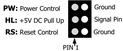
Top View of the System Panel and LED Connectors
